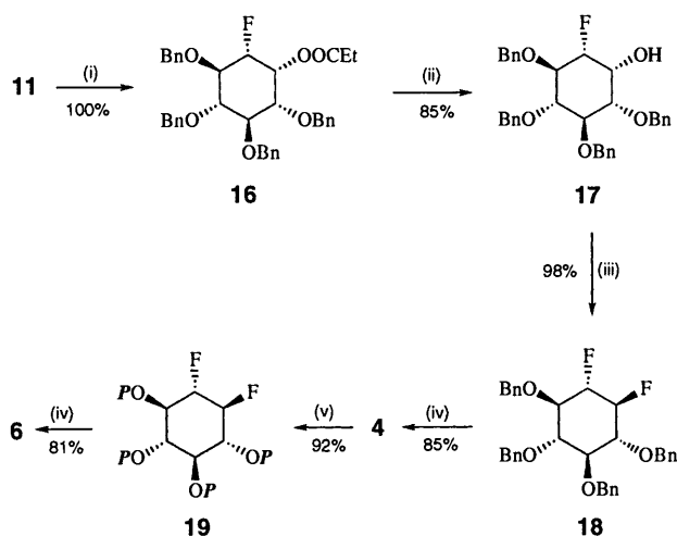
Scheme 3 Synthesis of DL-1,2-dideoxy-1,2-difluoro- scyllo -inositol 4 and its tetrakisphosphate 6 . P = (\text{BnO})_2\text{P}(\text{O})^- ; (i) \text{EtCO}_2^- \text{Cs}^+ , DMF; (ii) 5 M aq. NaOH, MeOH; (iii) DAST, \text{CH}_2\text{Cl}_2 ; (iv) \text{H}_2 , Pd-C; (v) (\text{BnO})_2\text{PNPr}^i_2 , then MCPBA.
